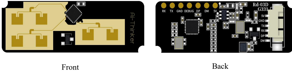
Figure 5 Pin diagram
