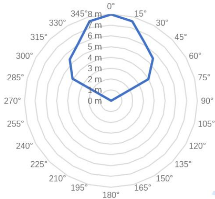
Figure 10 Schematic diagram of tracking range of wall mounting
