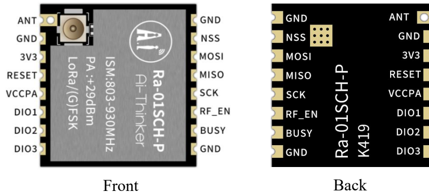
Figure 5 Pin diagram
