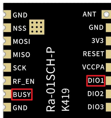
Figure 8 BUSY/DIO1 application considerations
