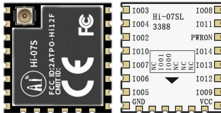
Figure 3 The appearance of the module(For reference only)
