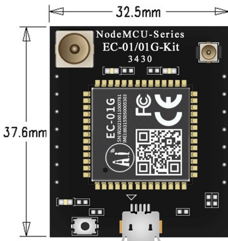
Figure 5 Development board size diagram
