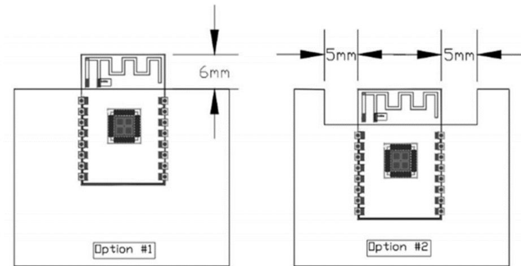
Figure 10 Schematic diagram of the antenna layout
