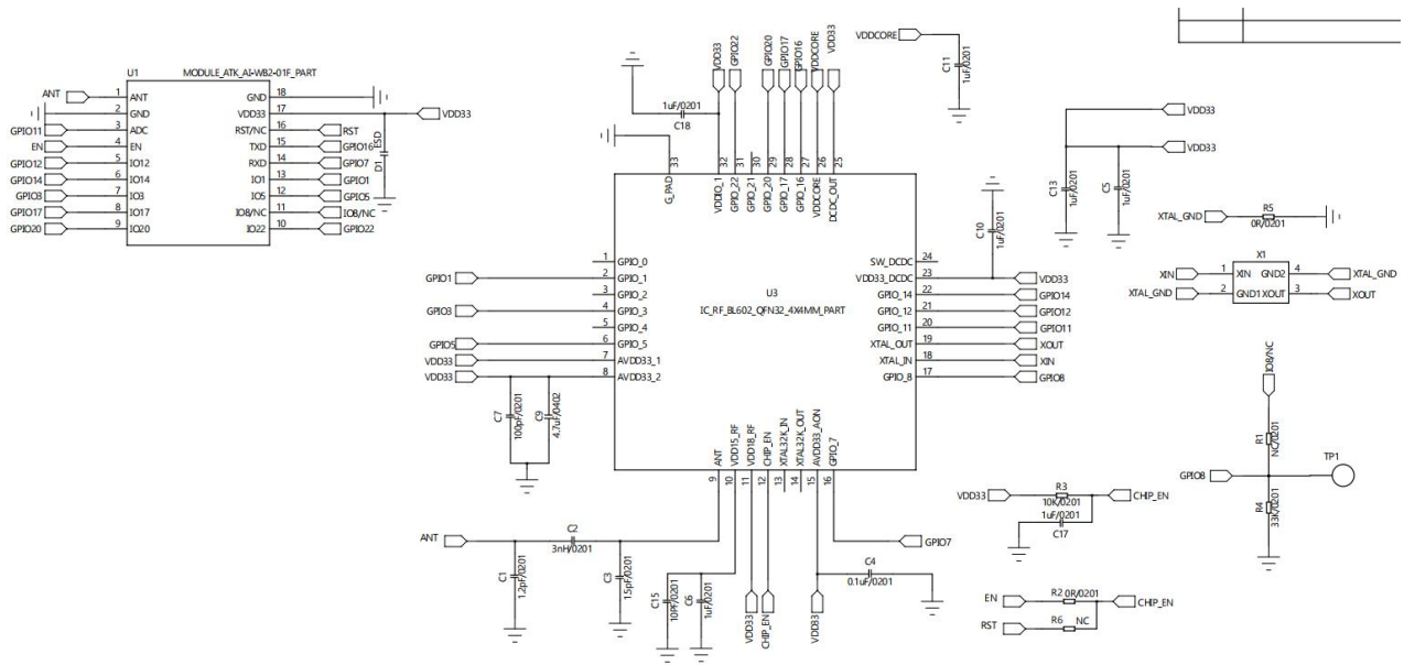
Figure 7 Module schematic
