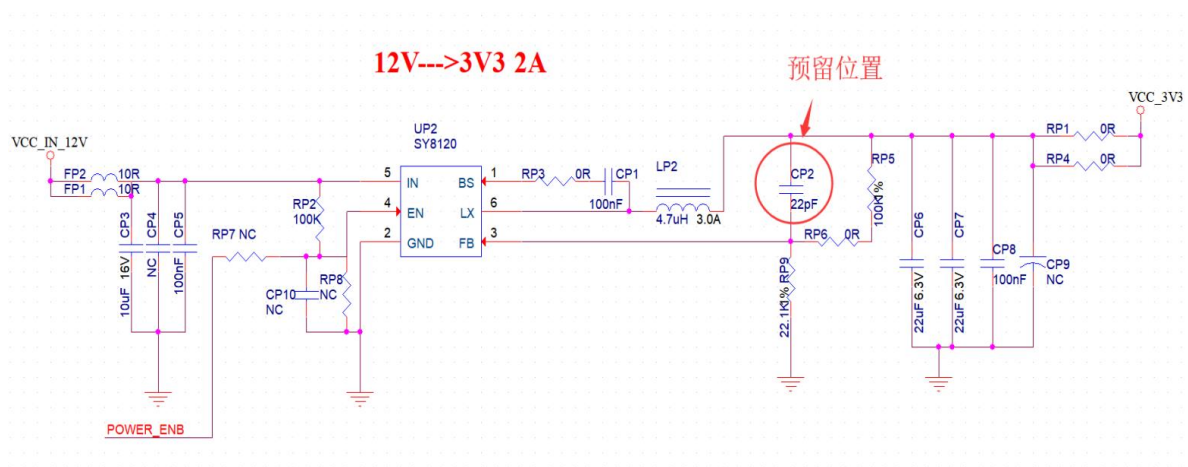
Figure 11 DC-DC step-down circuit diagram
