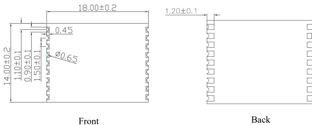
Figure 4 Dimension diagram
