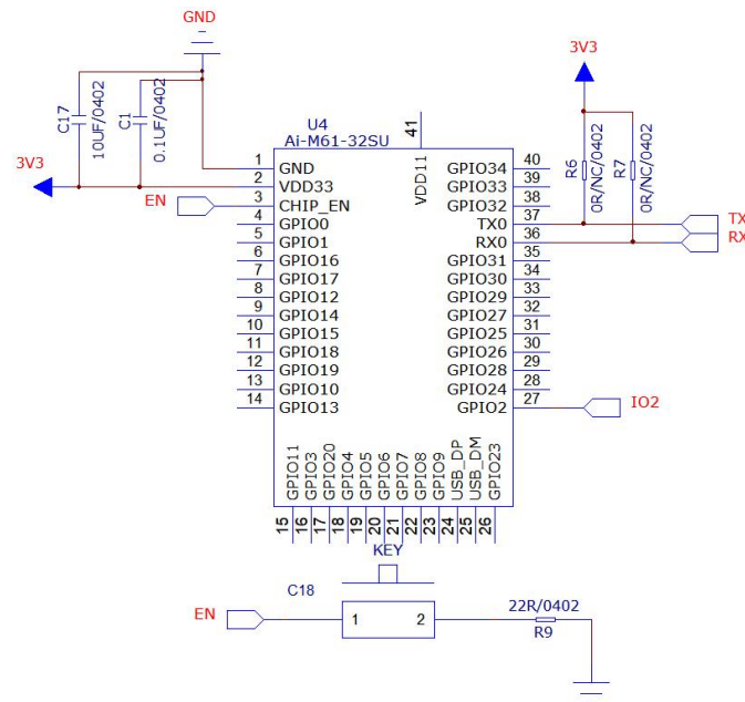
Figure 8 Application circuit diagram
